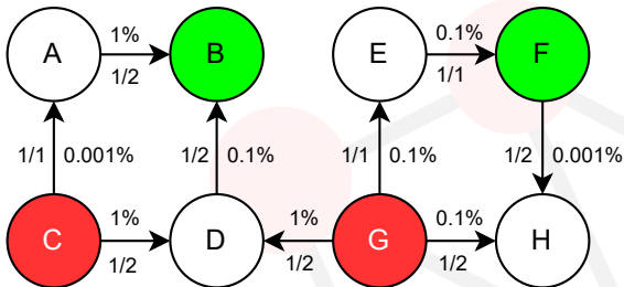
Figura 2: S_1 = \{B, F\} y PMI(S_1) = 3 .
