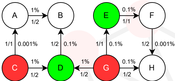
Figura 3: S_2 = \{E, D\} , PMI(S_2) = 1 .
